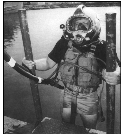
Figure 8-1. MK 21 MOD 1 SSDS.
